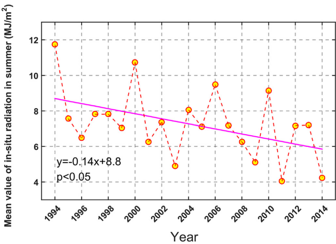
Fig. 8. Temporal variation of SLB-day averaged daily direct solar radiation reaching the surface at Shanghai site in each summer from 1994 to 2014. The temporal trend of the downwelling direct solar radiation was also shown in the pink line. (For interpretation of the references to colour in this figure legend, the reader is referred to the web version of this article.)
