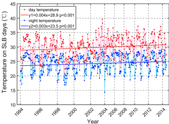
Fig. 7. Temporal variation of day (maximum value) and night (minimum value) near surface air temperature measured at Shanghai site on SLB days from 1994 to 2014. The linear regression lines are obtained based on yearly average temperature during day and night time, respectively.
